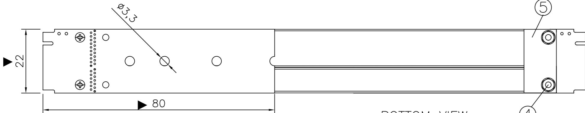
BOTTOM VIEW
